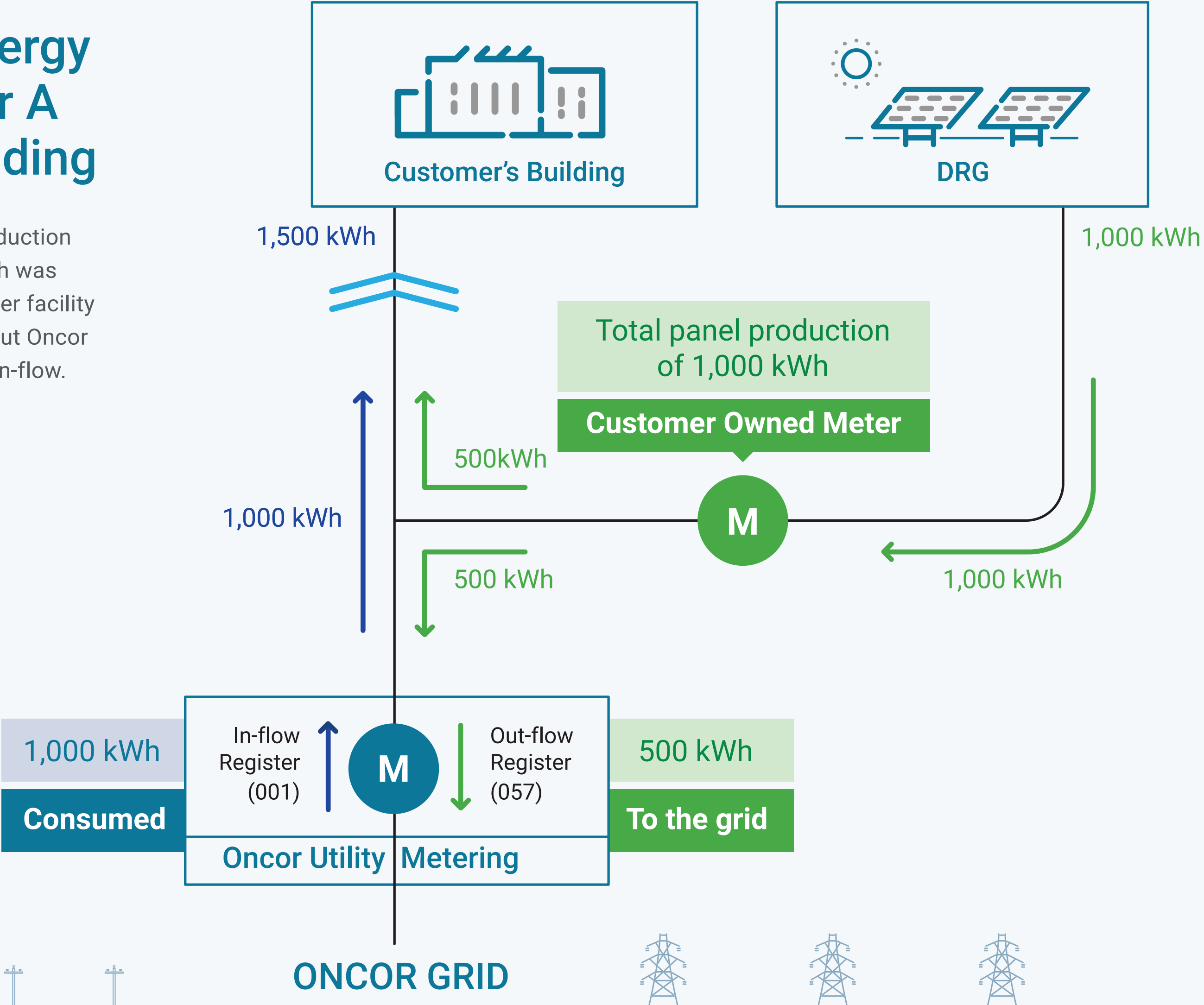
Figure 1 – Customer Metering Versus Oncor Metering
