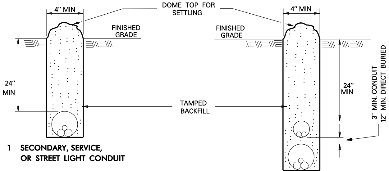
1 SECONDARY CONDUIT AND 1 STREET LIGHT CONDUIT VERTICALLY ARRANGED
