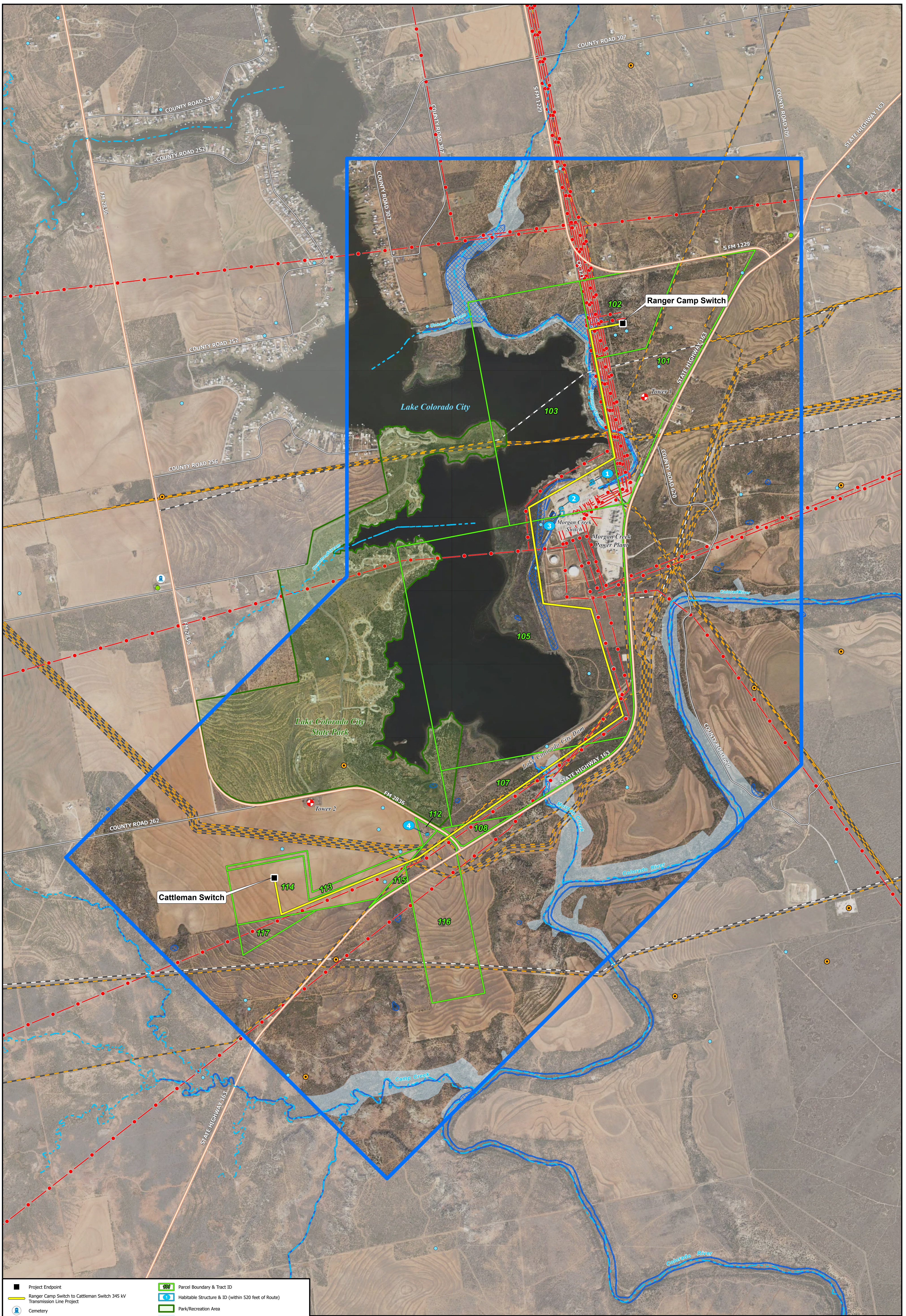
Figure 3-1 Environmental and Land Use Constraints Ranger Camp Switch to Cattleman Switch 345 kV Transmission Line Oncor Electric Delivery Company LLC Mitchell County, Texas
