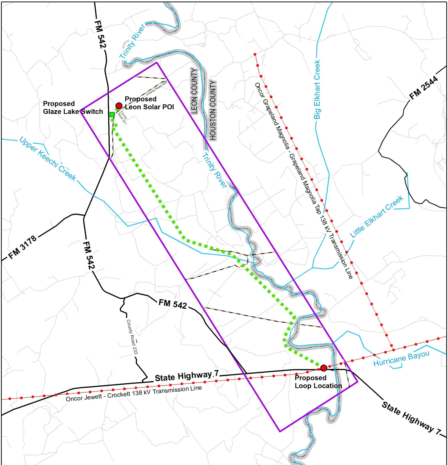
FIGURE 1. DETAILED ROUTE DESCRIPTION MAP GLAZE LAKE SWITCH 138 kV LOOP TRANSMISSION LINE PROJECT
